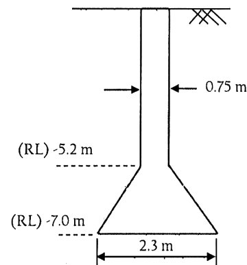
Proposed Belled Pier
