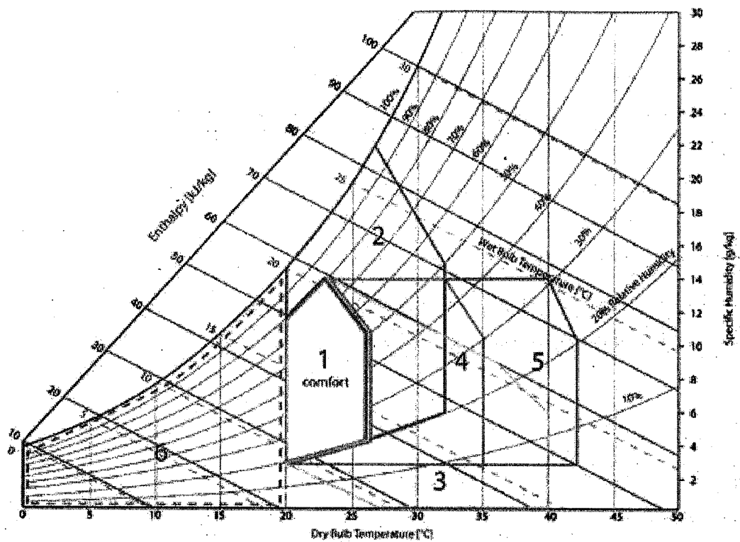
Givoni's bioclimatic chart
